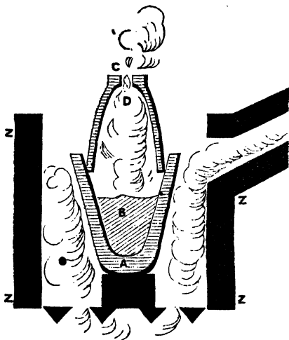
Fig. 226. Preparation of the Anhydrous Teroxide of Antimony. A. Lower crucible standing on a brick in the furnace z z z z, and containing the melted antimony B, which, being gradually oxidized, forms the teroxide; and this latter sublims into the upper inverted crucible, with hole in bottom, C, and condenses at D in needle-shaped crystals.
